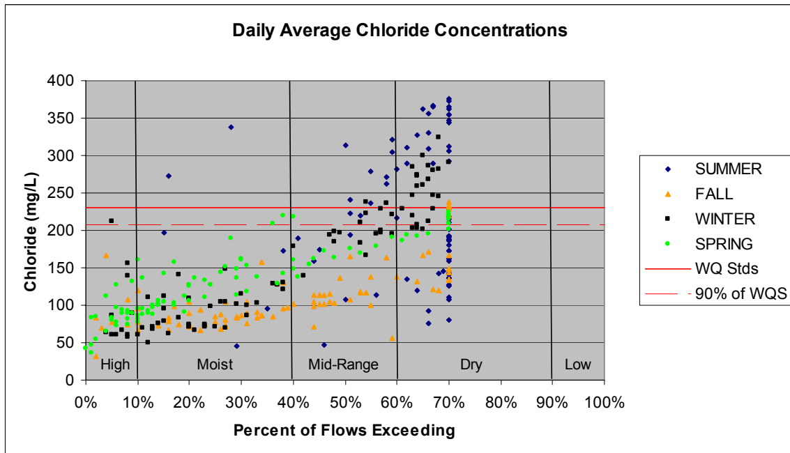
Figure 3: Concentration-Flow Duration Plot for Station I93-NTC-01
