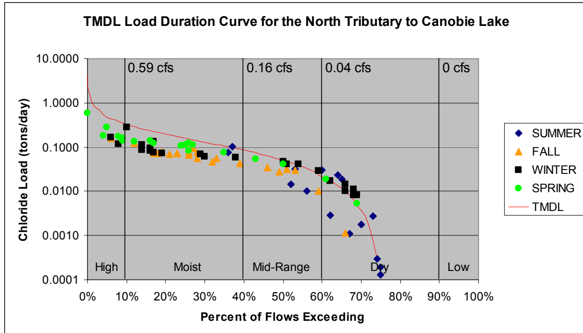
Figure 5: TMDL Load Duration Curve at Station I93-NTC-01
