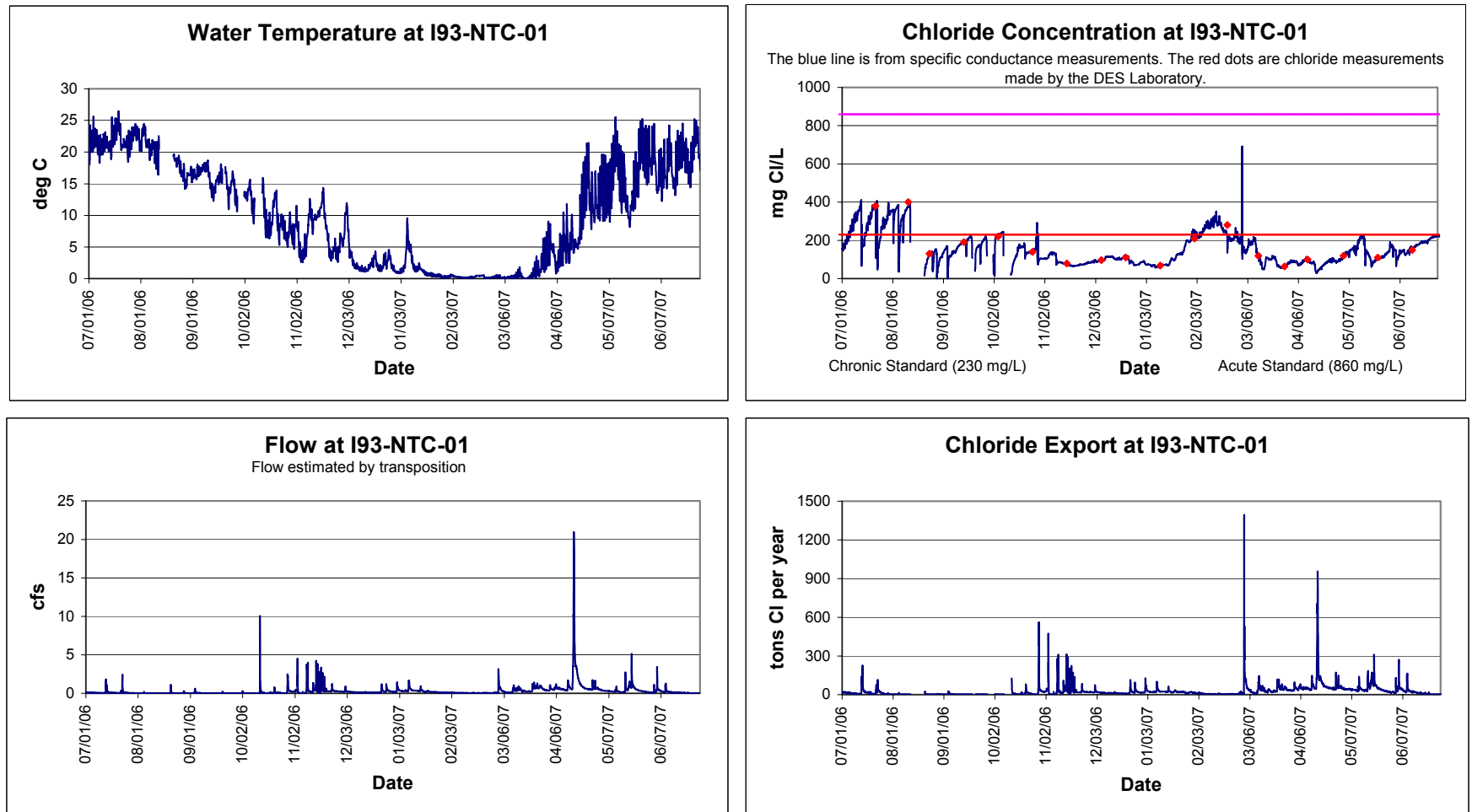
Figure 2: Time Series of Temperature, Chloride, Stream Flow and Chloride Export at Station I93-NTC-01
